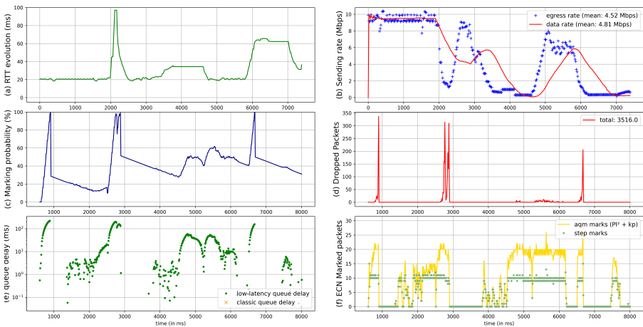
Fig. 7: Time series of impacts of a malformed (unpaced) flow on a legitimate low latency flow (router rate is set to 10Mbps). The vertical axes of the subfigures are the same measured metrics used for subfigures of the standard behavior (the first two show metrics from the legitimate endpoint, the others show metrics from the router) and the horizontal axis is the time in ms.
