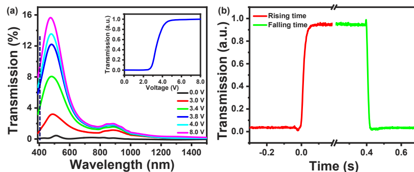
Fig. 4. (a) Optical transmission spectra as a function of the applied voltage for the nanoaperture array with W = 50 nm and P = 150 nm. Inset shows the normalized transmission versus applied voltage at the fixed wavelength of 400 nm marked with a vertical dash line in the spectra. (b) Experimentally measured rising and falling time at the applied voltage of 4.2 V.
