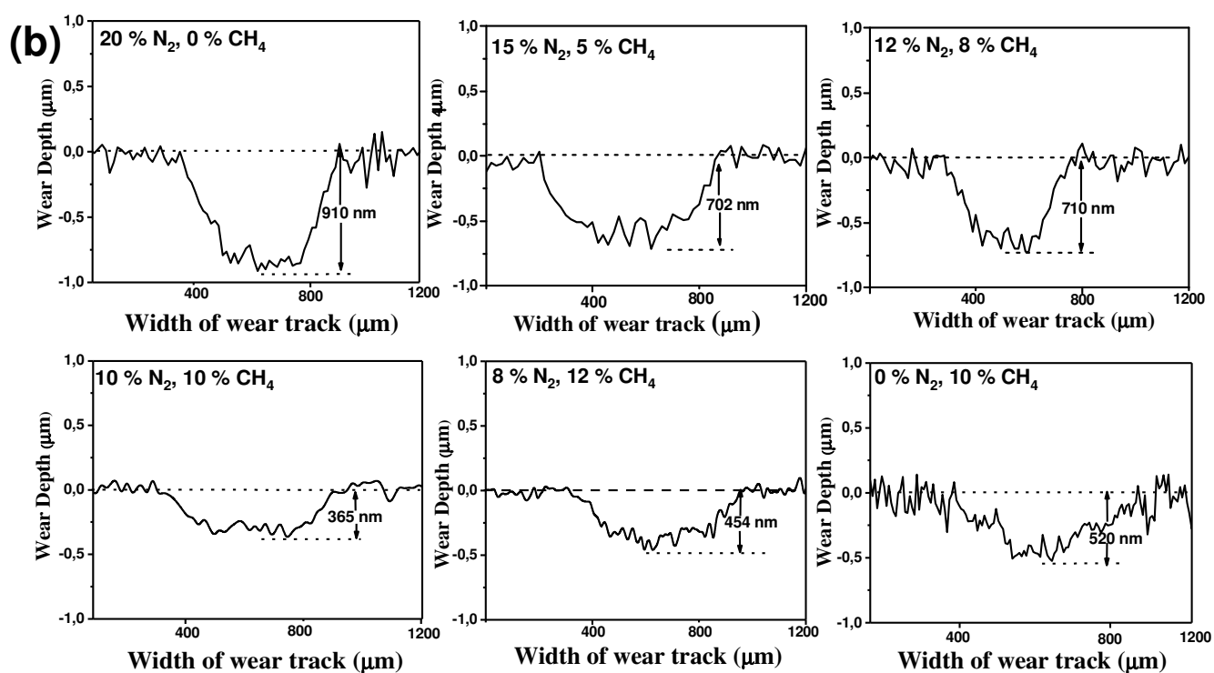
Fig. 9. Evolution of: a) wear rate and b) depth and width of wear tracks of Cr–V–C–N coatings deposited under different (N 2 and CH 4 ) flow rates.
