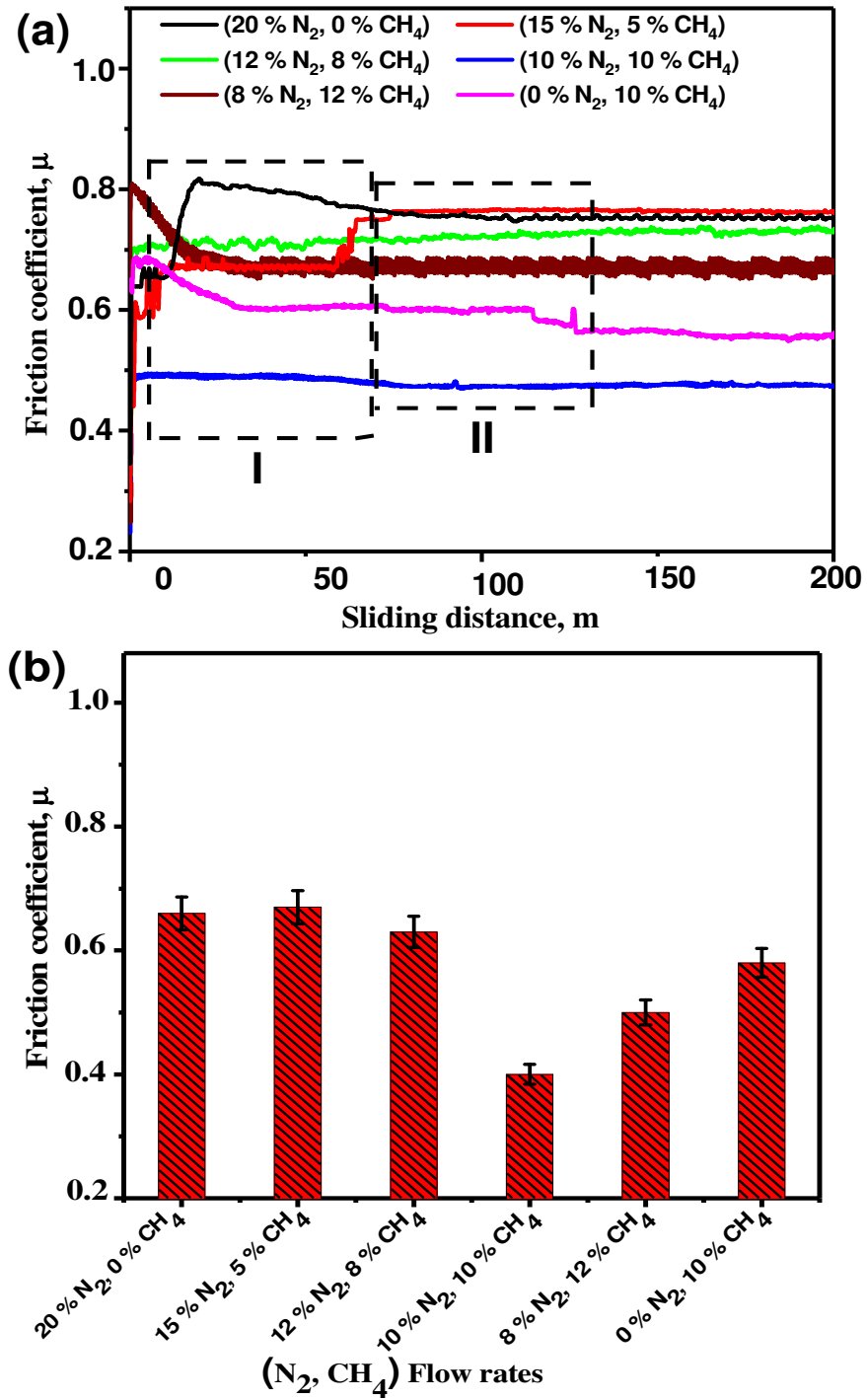
Fig. 8. Friction coefficients of Cr–V–C–N coatings as a function of: a) sliding distance, and b) ( \text{N}_2 and \text{CH}_4 ) flow rates.
