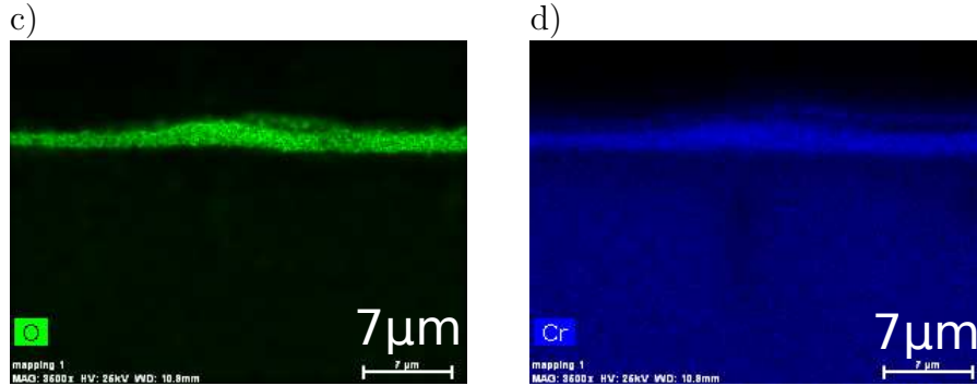
Figure 3: Chemical analysis of the cross-section of oxidized Ni38Cr for oxidation at 800°C during 3h: a) BSE cross-section; b) Ni content; c) O content; d) Cr content ; ellipse in red is the location of Cr depletion.
