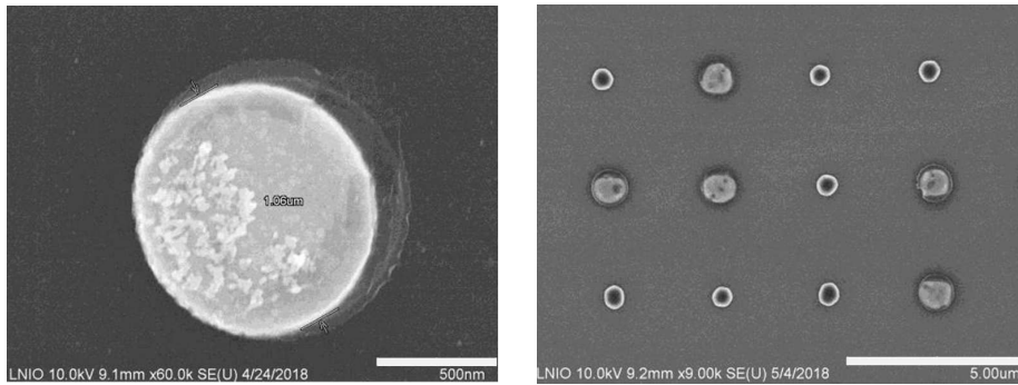
Figure 5: Evolution of Au particle at 900^{\circ}\text{C} during 30min in an inert environment (no oxidation occurs); left at room temperature (initial surface shape is a circle); right at 900^{\circ}\text{C} after 30min
