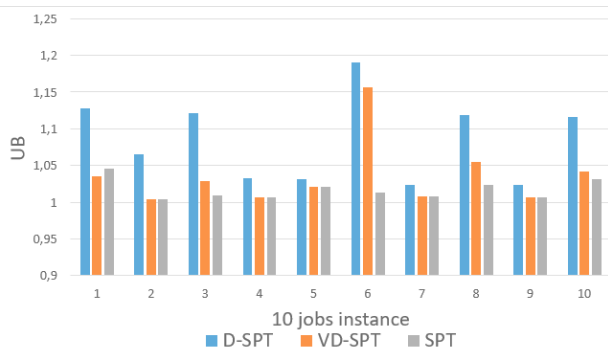
Fig. 3. Upper Bound on the competitive ratio for 10-jobs problem
