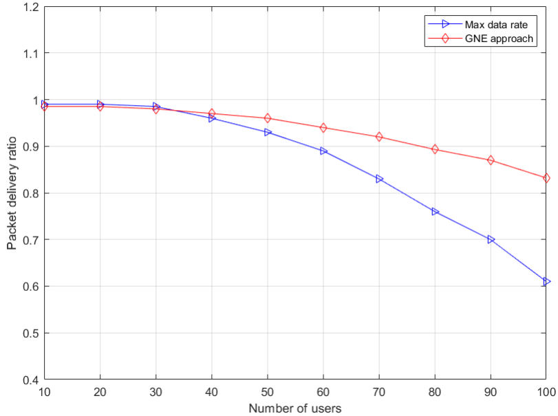
Figure 5: Packet delivery ratio versus the number of vehicles
