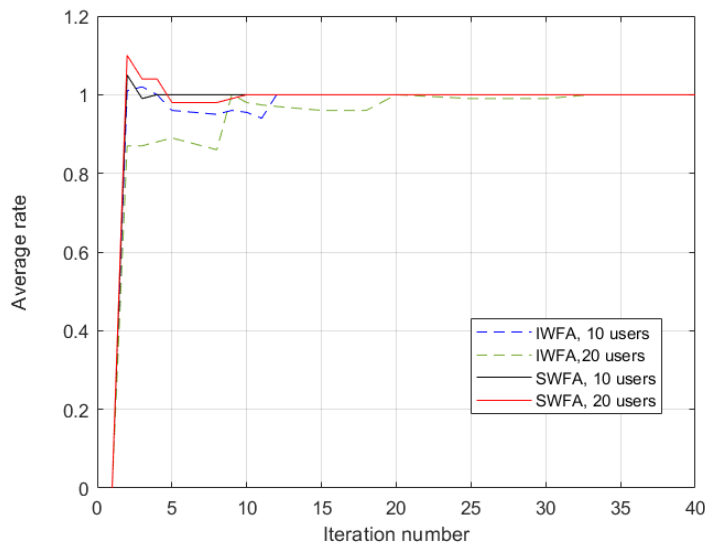
Figure 6: Convergence speed of IWFA and SWFA
