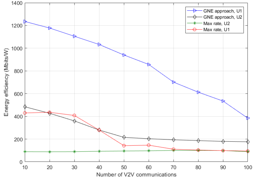
Figure 4: Energy efficiency vs. the number of V2V communications
