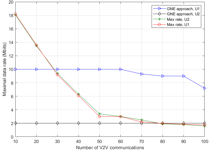
Figure 3: Impact of the number of V2V communications on the data rate.
