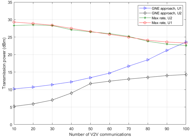
Figure 2: Impact of the number of V2V communications on the transmit power.
