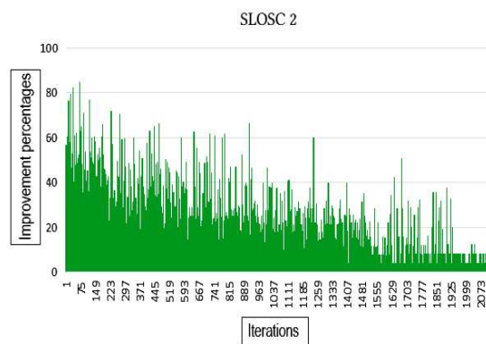
Figure 38: SLOSC 2 crossover operator.
