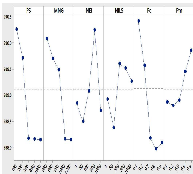
Figure 24: Main effect plot of means GA 1.
