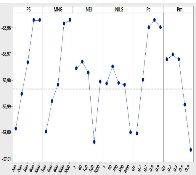
Figure 27: Main effect plot of S/N ratios GA 2.
