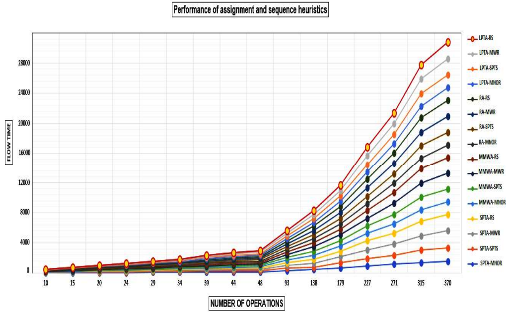
Figure 54: Performance of ILS 1 in terms of quality with the different combinations of heuristics for the generation of initial solutions.
