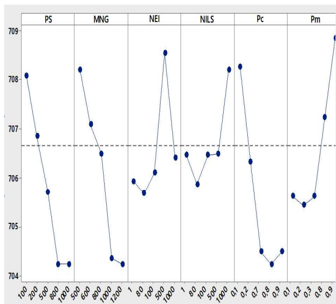
Figure 26: Main effect plot of means GA 2.
