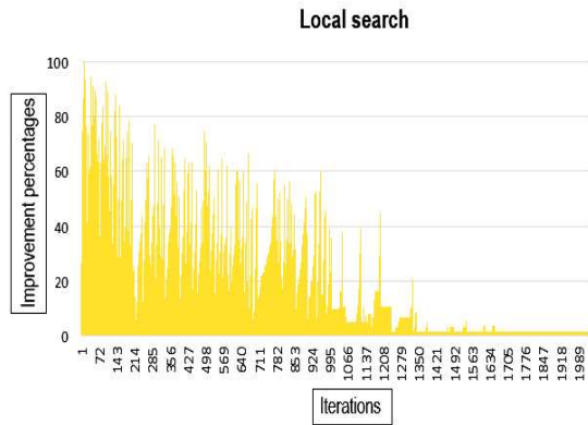
Figure 39: Local search with operators OMAC 1, JLOSC 1 and SLOSC 1.
