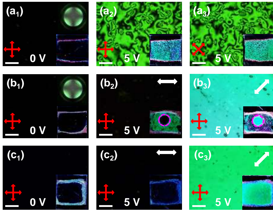
Figure 3. Polarized optical images of a pristine (a 1 –a 3 ), LPVL-treated (b 1 –b 3 ), UV-treated (c 1 –c 3 ) homeotropic cell at 0^\circ sample stage rotation with no driving voltage (a 1 , b 1 , and c 1 ), at 0^\circ sample stage rotation with the driving voltage of 5 V (a 2 , b 2 , and c 2 ), and at 45^\circ sample stage rotation with the driving voltage of 5 V (a 3 , b 3 , and c 3 ). The top right insets in 3a 1 and 3b 1 show the conoscopic image. All the bottom right insets illustrate the complete sample photos observed under two crossed polarizers. The scale bar at the bottom left corner in each image is 100 \mu\text{m} .
