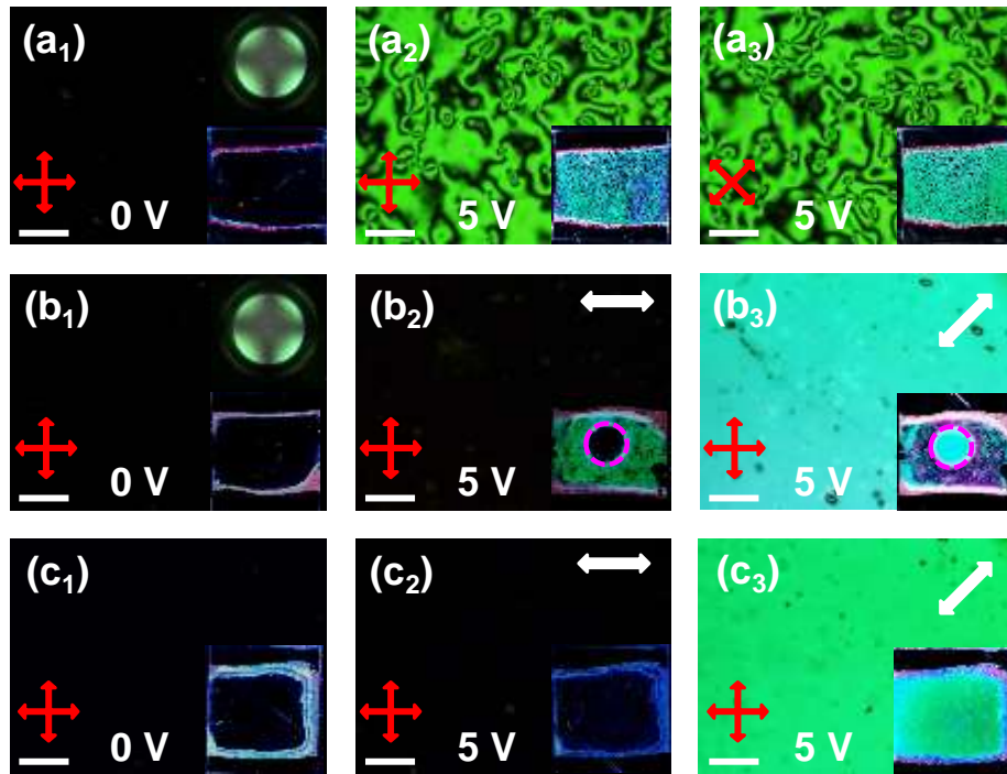
Figure 3. Polarized optical images of a pristine (a 1 –a 3 ), LPVL-treated (b 1 –b 3 ), UV-treated (c 1 –c 3 ) homeotropic cell at 0° sample stage rotation with no driving voltage (a 1 , b 1 , and c 1 ), at 0° sample stage rotation with the driving voltage of 5 V (a 2 , b 2 , and c 2 ), and at 45° sample stage rotation with the driving voltage of 5 V (a 3 , b 3 , and c 3 ). The top right insets in 3a 1 and 3b 1 show the conoscopic image. All the bottom right insets illustrate the complete sample photos observed under two crossed polarizers. The scale bar at the bottom left corner in each image is 100 μm.
