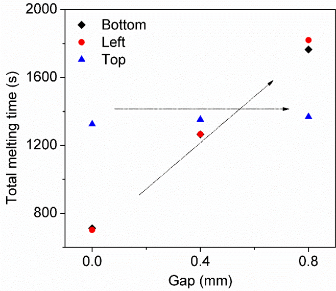
Fig. 11. Total melting time of composite PCM
