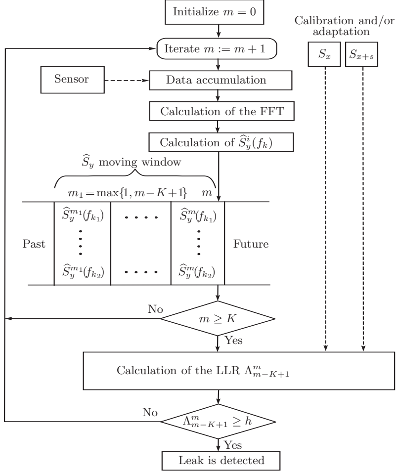
Figure 1: The flowchart of the leak detection algorithm. The flowlines show the process's order of operation and the dashed lines with arrowheads show the transmission of information.
