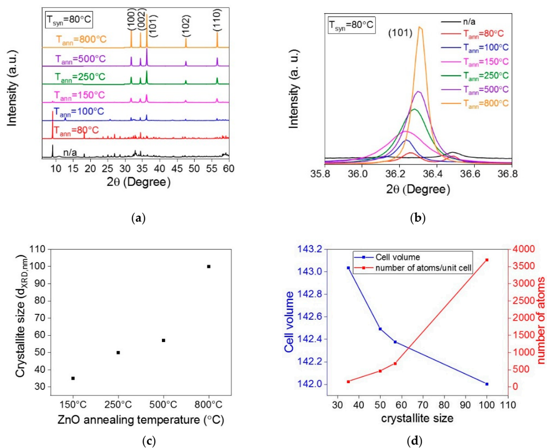
Figure 3. XRD measurements of the powdered ZnO nanoparticles (NP) synthesized at 80^\circ\text{C} and annealed at different temperatures: (a) XRD patterns, (b) the variation of the (101) plane peak intensity and position with increasing the annealing temperatures, (c) the evolution of the crystallite size as a function of annealing temperature, (d) the illustration of the variation of the cell volume and number of atoms per unit cell as a function of crystallite size.
