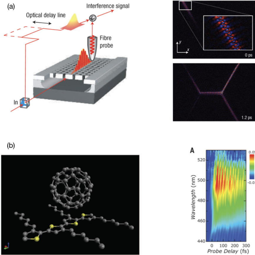
Figure 6: Spatiotemporally resolved investigation of energy and charge transfer. (a) Recording of pulse propagation in a nanophotonic wave guide structure based on spectral interference measurements resolving the nanoscale electrical field evolution (reprinted Fig. 2 and Fig. 3 with permission from Ref. [99]. Copyright (2007) by Springer Nature Publishing Group). (b) Charge transfer dynamics in the P3HT:PCBM blend. The left part shows the Molecular structure of the P3HT:C60 compound. In the right panel the transient differential absorption signal reveals the photon induced charge transfer from the the polymer to the fullerene that is facilitated by the coherent oscillations seen in the transient signal. (reprinted Fig. 1c and Fig. 2a with permission from Ref. [105]. Copyright (2014) by the American Association for the Advancement of Science).
