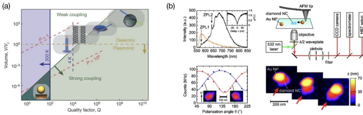
Figure 5: (a) The quality factor, Q , of nanoantennas is plotted against its effective volume, V/V_\lambda showing strong-coupling (green arrow), room-temperature (blue arrow), and plasmonic (orange arrow) regimes for single emitters (reprinted Fig. 1a with permission from Ref. [78]). Copyright (2016) by the Springer Nature Publishing Group). (b) Optical properties and nanoscale manipulation of diamond nanocrystals and gold nanoparticles. The gold sphere is moved around the diamond nanocrystal, which stays fixed in its orientation, thus testing the optimal configuration for emission enhancement (reprinted Fig. 1 with permission from Ref. [90]). Copyright (2009) by the American Chemical Society).
