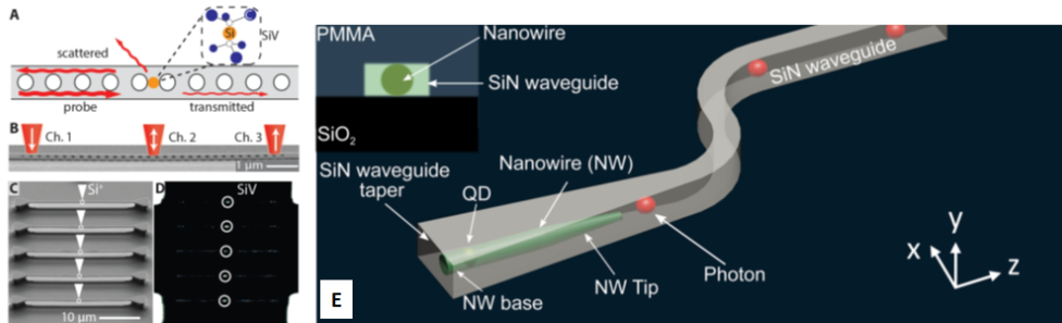
Figure 3: (a) Schematic of a single SiV color center in a diamond photonic cavity. (b) Scanning electron micrograph (SEM) of such a diamond photonic crystal. (c) SEM of diamond cavities fabricated without color centers. (d) SiV fluorescence for each nanocavity after focused Si + ion beam implantation to create the color centers. (reprinted Fig. 1a-d with permission from Ref. [13]. Copyright (2016) by the American Association for the Advancement of Science). (e) Schematic view of a III-V QD in a nanowire embedded in a Si 3 N 4 photonic waveguide after micro-manipulation (reprinted Fig. 1a with permission from Ref. [63]. Copyright (2016) by the American Chemical Society).
