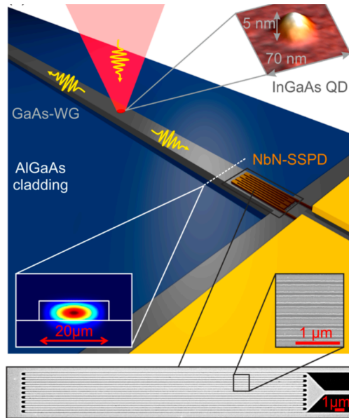
Figure 2: Integration of a QD single-photon emitter with on-chip superconducting single-photon detector. Schematic of a 2-mm-long GaAs ridge waveguide containing a single layer of InGaAs QDs. The dots are excited by a free-space pulsed laser diode and emit in the waveguide. The waveguide then propagates light towards an evanescently coupled NbN superconducting single-photon detector (reprinted Fig. 1 with permission from Ref. [48]. Copyright (2015) by the American Chemical Society).
