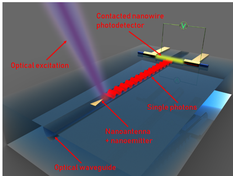
Figure 1: Schematic view of a fully integrated quantum circuit with an optical waveguide guiding single photons emitted efficiently from a nanoemitter coupled to a nanoantenna. The photons are then sent to a nanosystem photosensor for detection.
