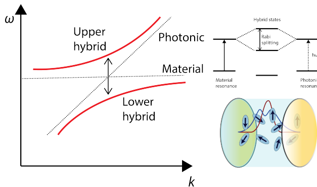
Figure 12: The strong interaction between the material entity and light within plasmonic/photonic cavities creates new hybrid lightmatter states that have significantly different energy levels from those of the material entity and of the optical system individually (adapted Fig. 1 with permission from Ref. [165]. Copyright (2018) by Wiley-VCH Verlag GmbH & Co. KGaA).
