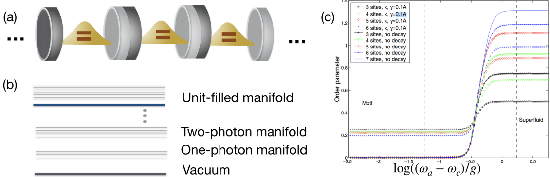
Figure 15: The Jaynes-Cummings-Hubbard model. (a) A sketch of a coupled cavity array, implementing the Jaynes-Cummings-Hubbard model. (b) Energy spectrum of the JCH model. (c) The order parameter Var(N_i) of the lowest-energy state in the unit-filled manifold as a function of detuning (\omega_a - \omega_c)/g for 3-7 sites with and without decay. The order parameter exhibits a jump from zero to a finite value, corresponding to the Mott and the superfluid phase, respectively. The transition gets a sharper width as the system's size is increased as expected from quantum phase transition (reprinted Fig. 2 with permission from Ref. [192]. Copyright (2007) by the American Physical Society).
