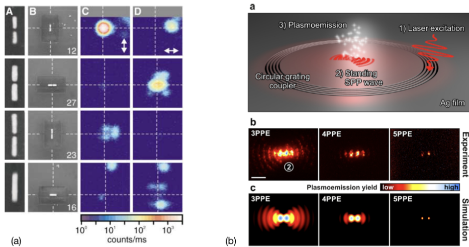
Figure 4: Nonlinear processes in nanoplasmonics. (a) Demonstration of the resonant interaction between optical nanoantennas shown as SEM micrographs in A and B. First and second row show confocal images of resonant white light generation for two incident polarizations indicated by white arrows, whereas third and fourth row show the non-resonant case. In the resonant case the nonlinear yield is enhanced by about 4 orders of magnitude (reprinted Fig. 1 with permission from Ref. [68]. Copyright (2005) by the American Association for the Advancement of Science). (b) The upper part visualizes the generation of focusing surface plasmon polaritons in a circular plasmon corral that leads to a multi-plasmon electron emission from the center of the corral. The lower two rows show measured and simulated emission patterns for different order multi-plasmon electron emission channels. (reprinted Fig. 3 with permission from Ref. [80]. Copyright (2017) by the American Chemical Society).
