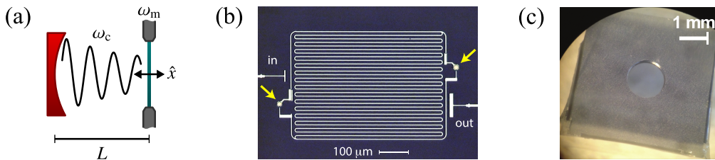
Figure 16: (a) The prototypical optomechanical system, consisting of a single mode of the electromagnetic field in a cavity of length L and resonance frequency \omega_c , one of whose end mirrors is allowed to move. The motion of this mirror is characterised by its oscillation frequency \omega_m and position operator \hat{x} . Further details are in the text. (b) A realisation of an optomechanical system with two moving elements as a superconducting LC circuit (reprinted Fig. 1a with permission from Ref. [200]. Copyright (2018) by the Springer Nature Publishing Group). (c) A macroscopic membrane, which may be placed inside an optical cavity to realise the optomechanical Hamiltonian (reprinted Fig. 8 with permission from Ref. [201]. Copyright (2017) by the Institute of Physics Publishing Ltd.).
