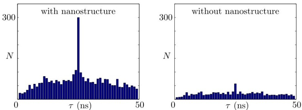
Figure 11: Coincidence peaks. Coincidence peaks obtained after one photon of the entangled pair is transferred through either the plasmonic structure at normal incidence (left) or a flat gold film (right) (reprinted Fig. 4 with permission from Ref. [168]. Copyright (2015) by Walter de Gruyter GmbH).
