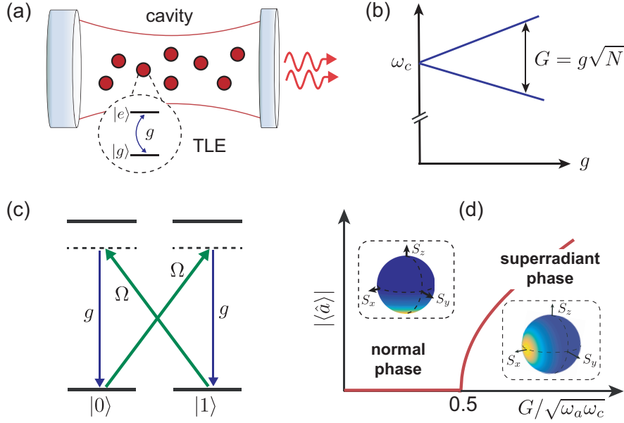
Figure 14: (a) Sketch of a CQED system with multiple two-level emitters (TLE) coupled to a single optical mode. (b) Collective effects give rise to enhanced light-matter interactions, which result, for example, in a frequency splitting G = g\sqrt{N} between the two lowest polariton modes formed by a superposition of a single photon and the collective state |S\rangle . (c) Two ground states |0\rangle and |1\rangle of an atom can be coupled to a cavity via Raman transitions involving additional laser fields with Rabi frequency \Omega . This technique can be used to engineer effective Dicke models with tunable parameters G , \omega_c and \omega_a [183]. (d) Above a certain coupling strength, the ground state of the Dicke model undergoes a phase transition from a normal phase without any photons to a superradiant phase with a non-vanishing field expectation value, \langle \hat{a} \rangle \neq 0 . At the same time the emitters are polarized along the x -direction, as indicated by the Bloch-sphere representation of the collective spin state.
