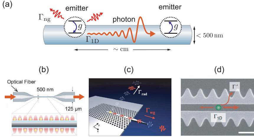
Figure 13: (a) Sketch of a waveguide QED setup with two quantum emitters coupled to a 1D photonic channel. If the rate of emission into the waveguide, \Gamma_{1D} , exceeds the emission rate \Gamma_{ng} into other, non-guided modes, efficient long-range interactions between multiple emitters can be attained. This 1D regime of light-matter interactions can be implemented, for example, with (b) trapped atoms coupled to the evanescent field of a tapered nanofiber (reprinted Fig. 1 with permission from Ref. [174]. Copyright (2011) by the American Physical Society), (c) QDs coupled to a photonic-crystal waveguide (reprinted Fig. 1a with permission from Ref. [175]. Copyright (2014) by the American Physical Society), or (d) by combining cold atoms and nanophotonic crystal structures in a so-called alligator waveguide setup (reprinted Fig. 1a with permission from Ref. [176]. Copyright (2014) by the Springer Nature Publishing Group).
