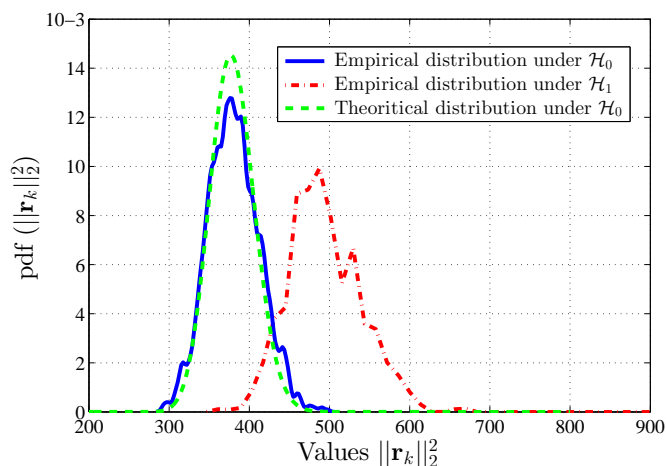
Figure 14: Empirical and theoretical distributions of normalized residuals norm for images with and without defect
