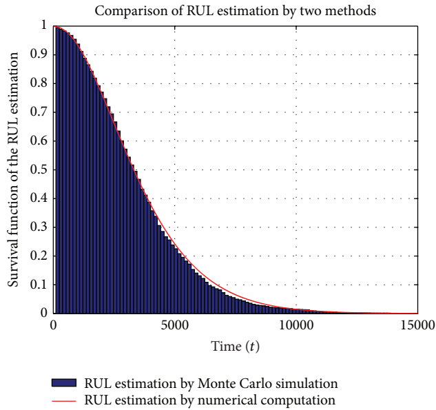
FIGURE 11: Comparison of the Remaining Useful Lifetime estimation of the water tank level control system at time T_{\text{prog}} = 15046.8 time units by two methods: Monte Carlo simulation and numerical computation using the estimated pdf of system state.
