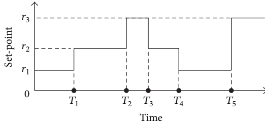
FIGURE 2: An example of set-point evolution.
