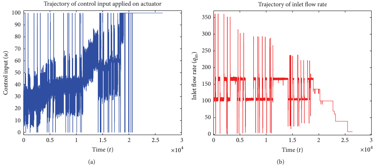
FIGURE 7: Control value applied on the actuator (a) and corresponding inlet flow rate (b).
