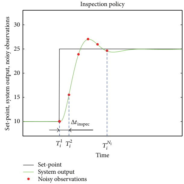
FIGURE 3: Inspection policy.
