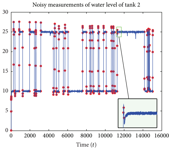
FIGURE 8: Noisy observations of water level of tank 2.
