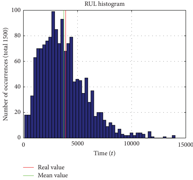
FIGURE 10: Remaining Useful Lifetime of the water tank level control system at time T_{\text{prog}} = 15046.8 time units.
