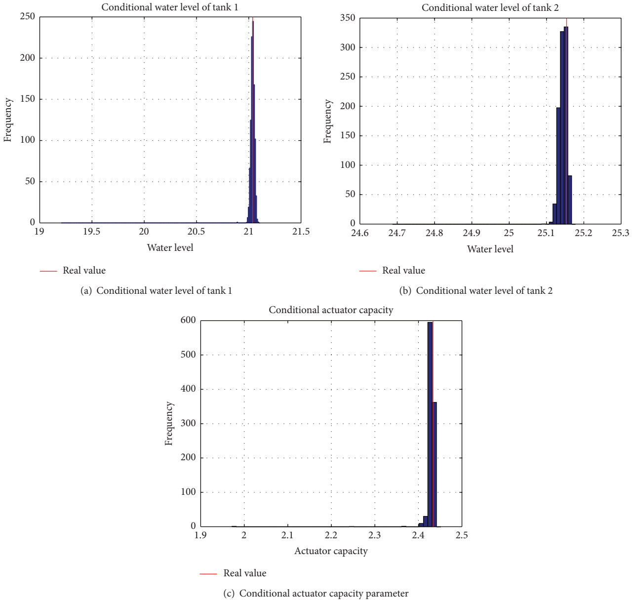
FIGURE 9: Conditional distribution of the system state at time T_{\text{prog}} = 15046.8 time units given the noisy measurements of h_2 for N_s = 1000 particles.
