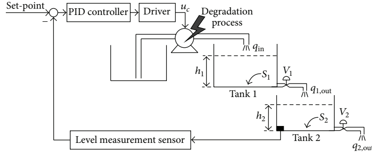
FIGURE 5: A double-tank level control system.
