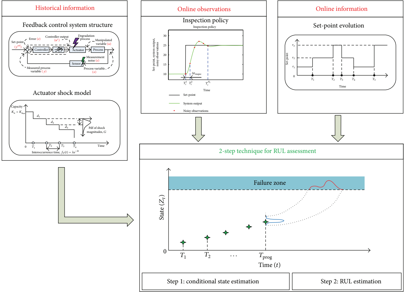
FIGURE 4: Illustration of the prognosis concept.
