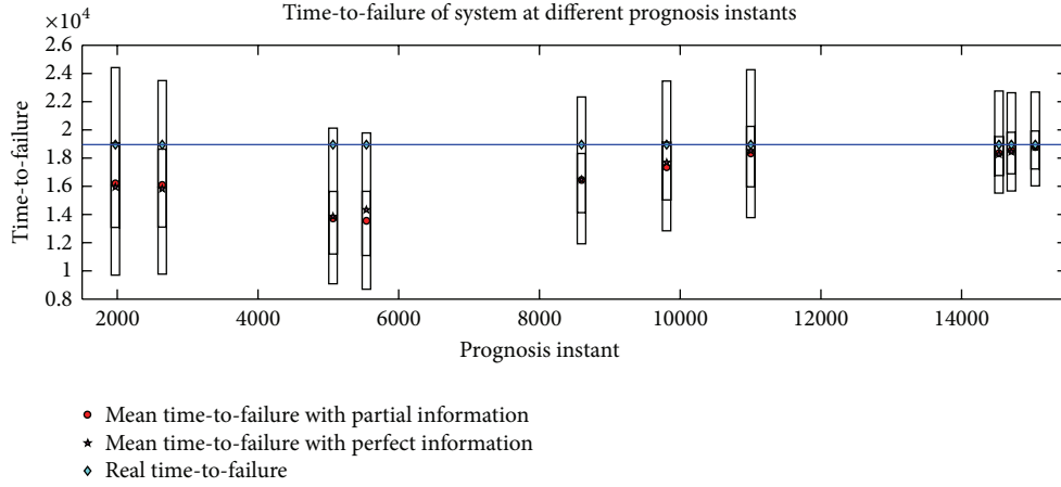
FIGURE 13: Mean time-to-failure (MTTF) in two cases of monitoring information at some different prognosis instants.
