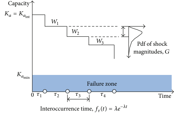
FIGURE 12: Cumulative damage model of actuator.
