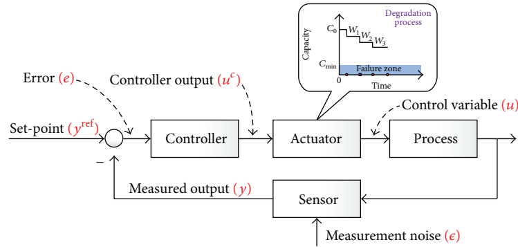
FIGURE 1: General block diagram of a feedback control system with notations.
