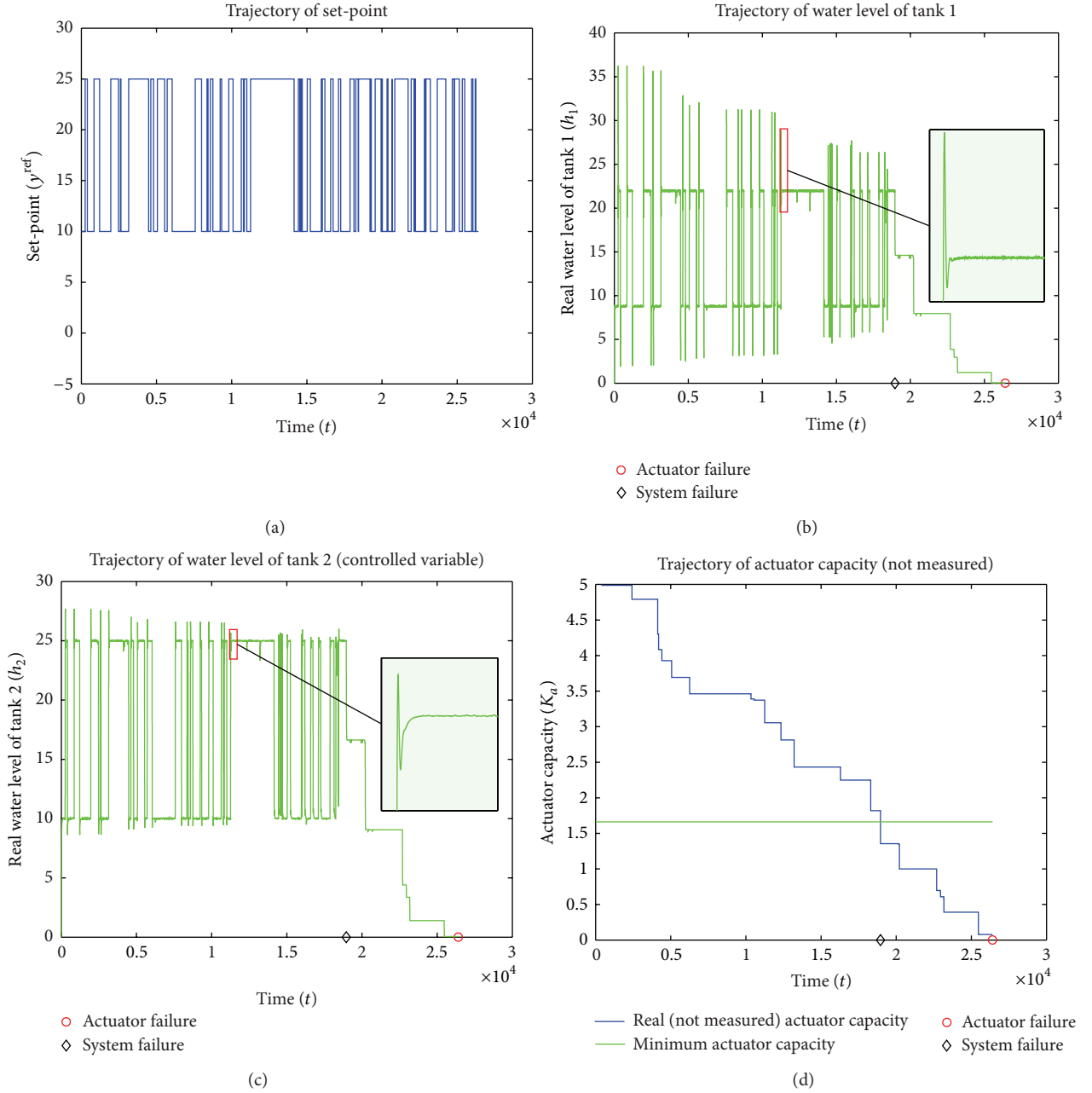
FIGURE 6: A trajectory of the water tank level control system until failure of actuator: (a) set-point, (b) water level of tank 1, (c) water level of tank 2, and (d) actuator capacity.
