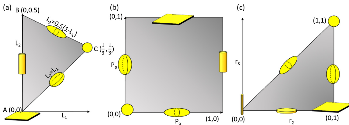
Fig. 1. Schematic representation of (a) L^2 , (b) P^2 and (c) r^2 spaces. The locus of spherical, prolate, oblate, cylinder NPs are reported in all spaces.
