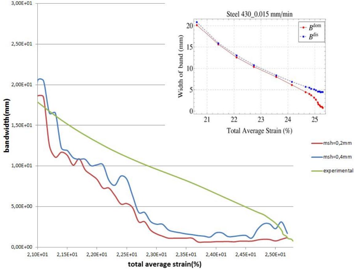
Figure 15. Evolution of the localization dominant band for (\bar{H} = 100, \bar{H}^g = 36) , numerical-experimental comparison for two varying meshes msh = 0,2\text{ mm} and msh = 0,4\text{ mm}
