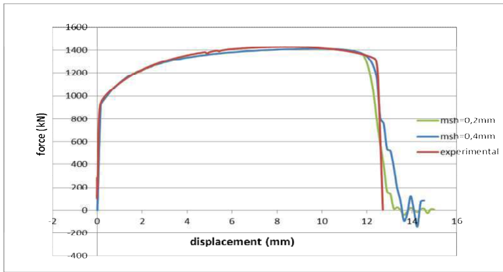
Figure 12. Comparison of the force-displacement curves for the two different mesh sizes.
