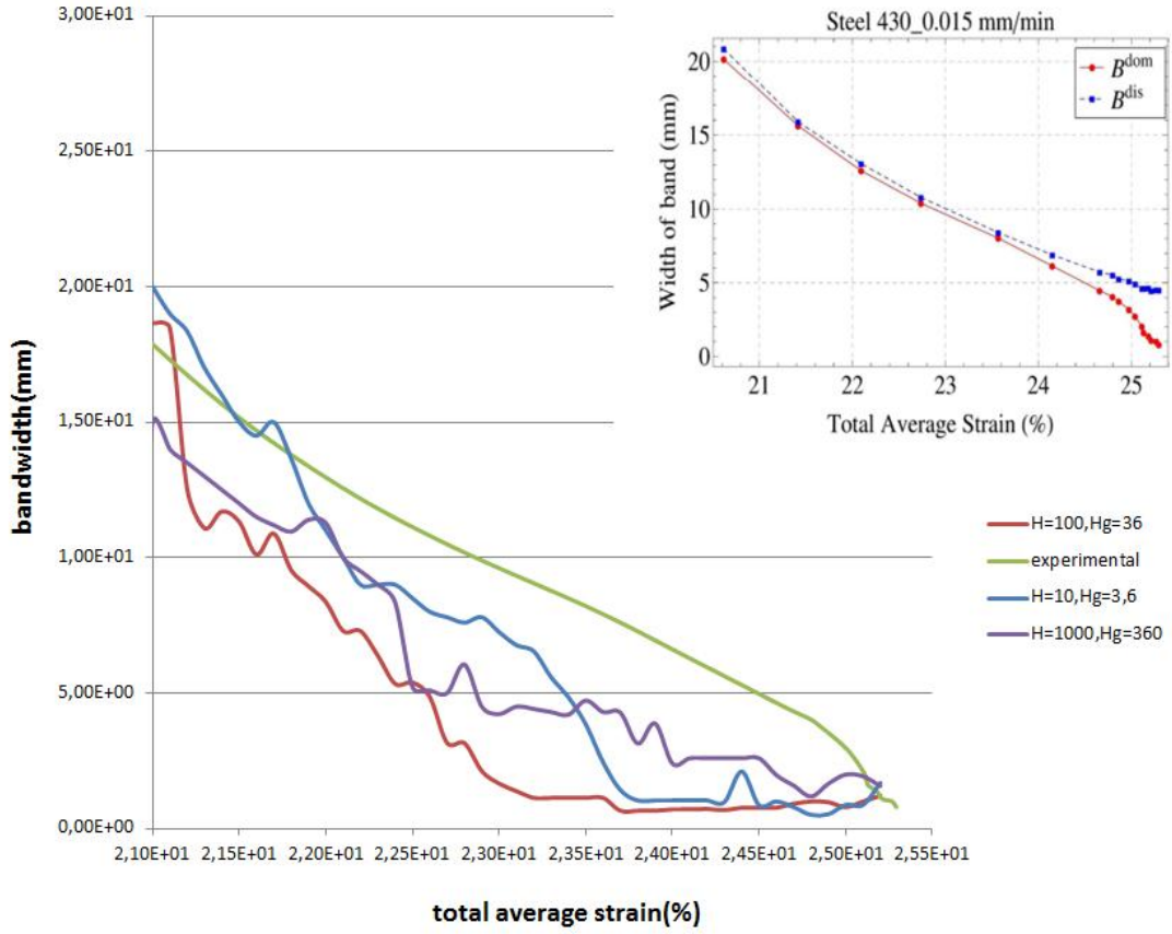
Figure 14. Evolution of the localization dominant band for a fixed mesh size, numerical-experimental comparison for (\tilde{H} = 10, \tilde{H}^g = 3,6) , (\tilde{H} = 100, \tilde{H}^g = 36) and (\tilde{H} = 1000, \tilde{H}^g = 360)
